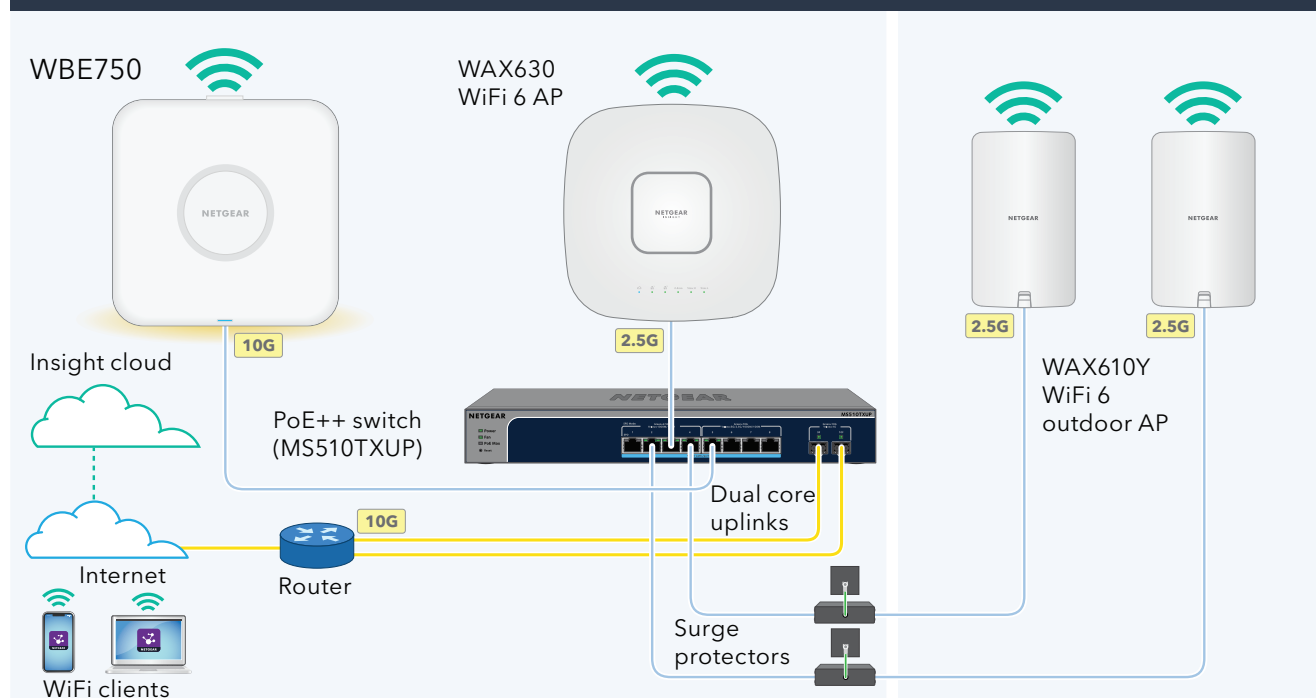
WBE750 Deployment Scenario
