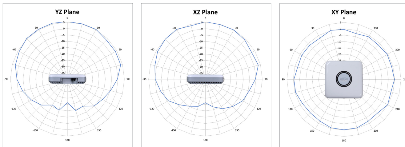
Radio Pattern for 6GHz
