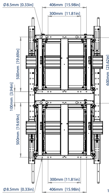
REAR VIEW
